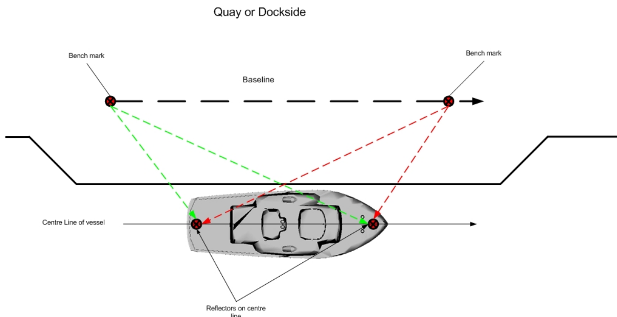
Figure 1: Gyrocompass Calibration method 1
